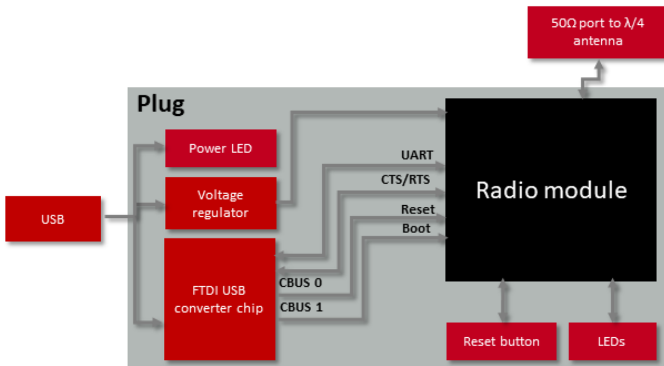
Figure 1: Block diagram of the Metis-e USB radio stick
